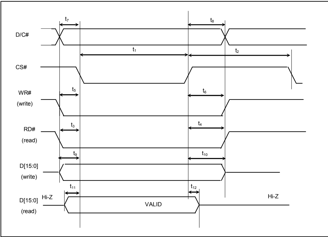
Figure 10-3 : 8080 Interface Timing
