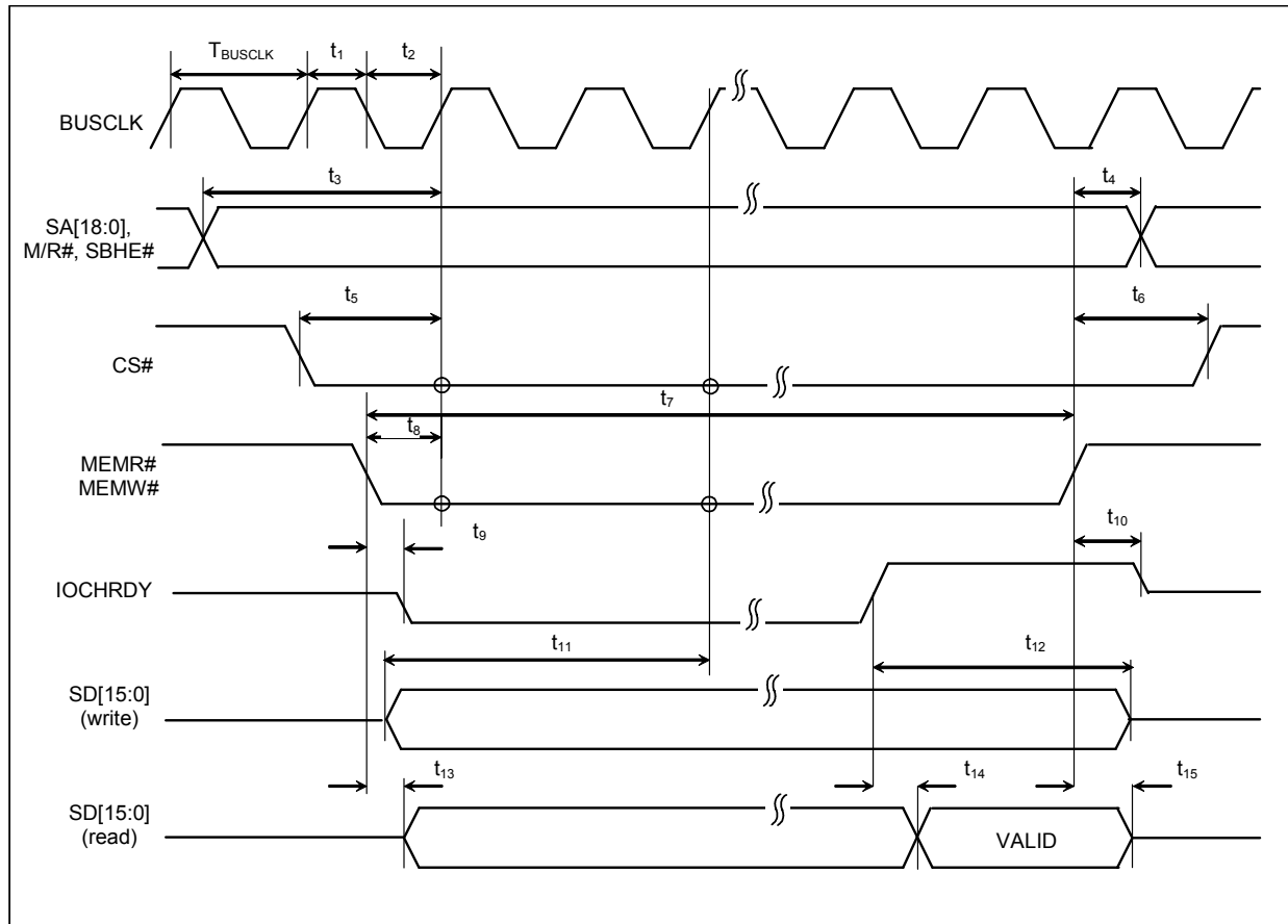
Figure 10-2 : Generic #2 Interface Timing
