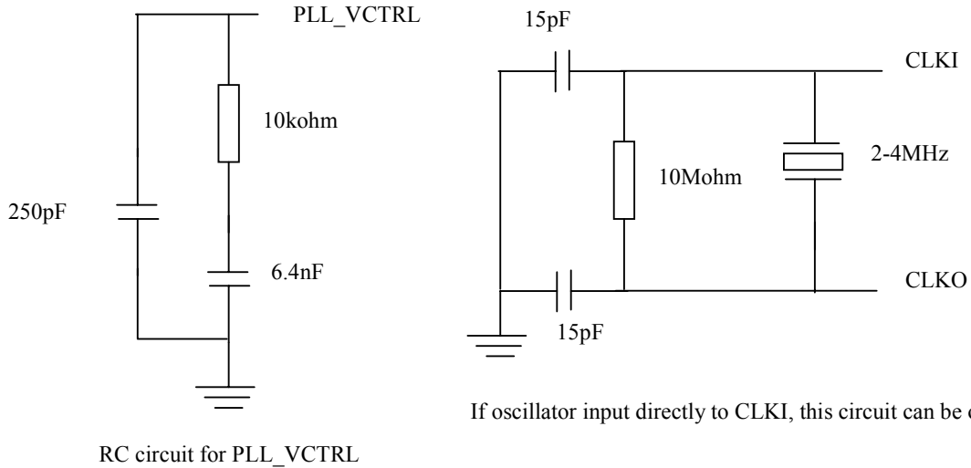
Figure 7-1 : Circuit for PLL enable
