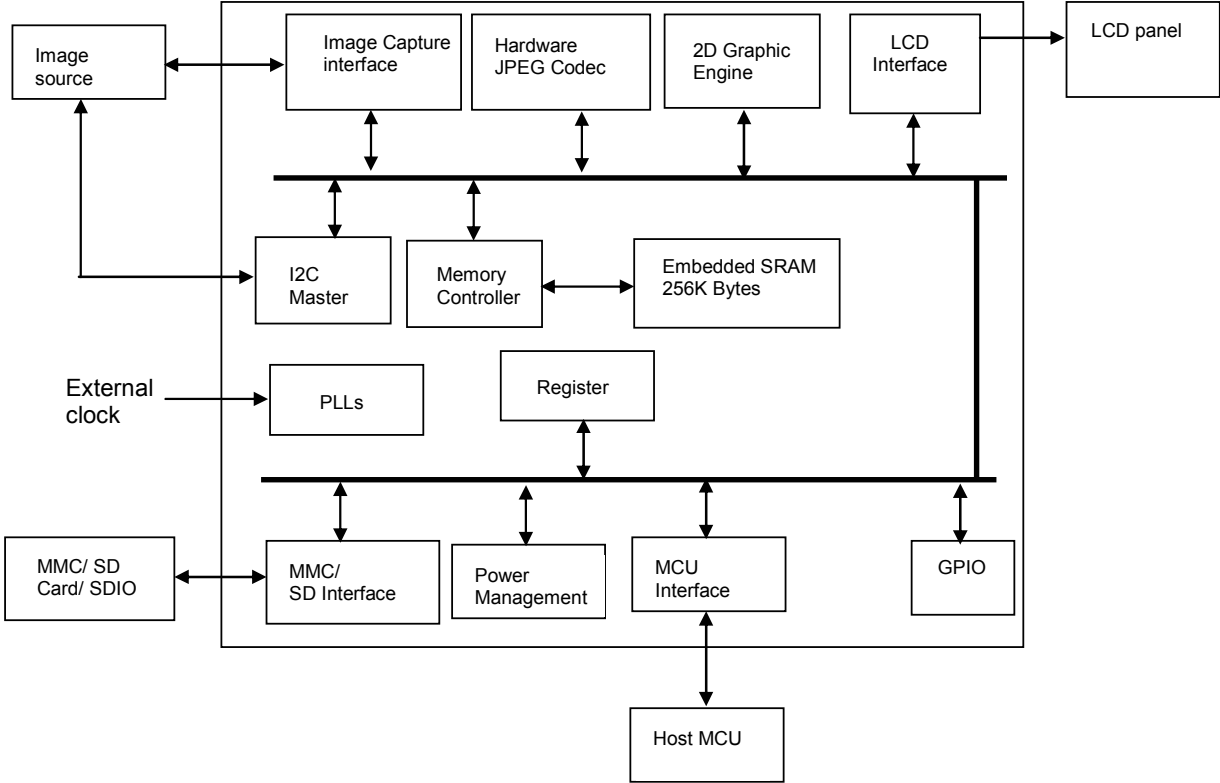
Figure 4-1 : SSD1928 Block Diagram
